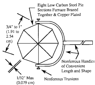
FIG. 14 Magnetic Field Indicator
